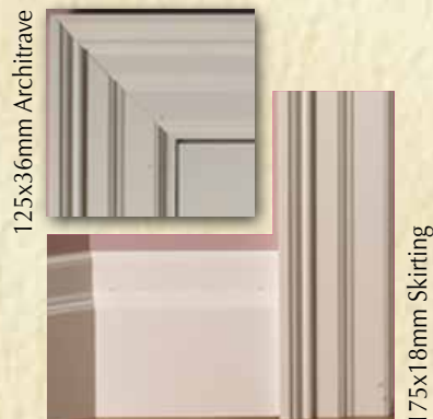
2 Part Architrave
